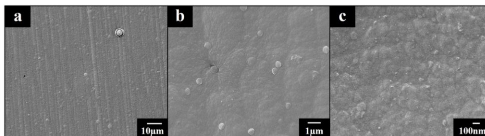
Fig. 9 SEM images of PPy coated stainless steels at different magnifications.
