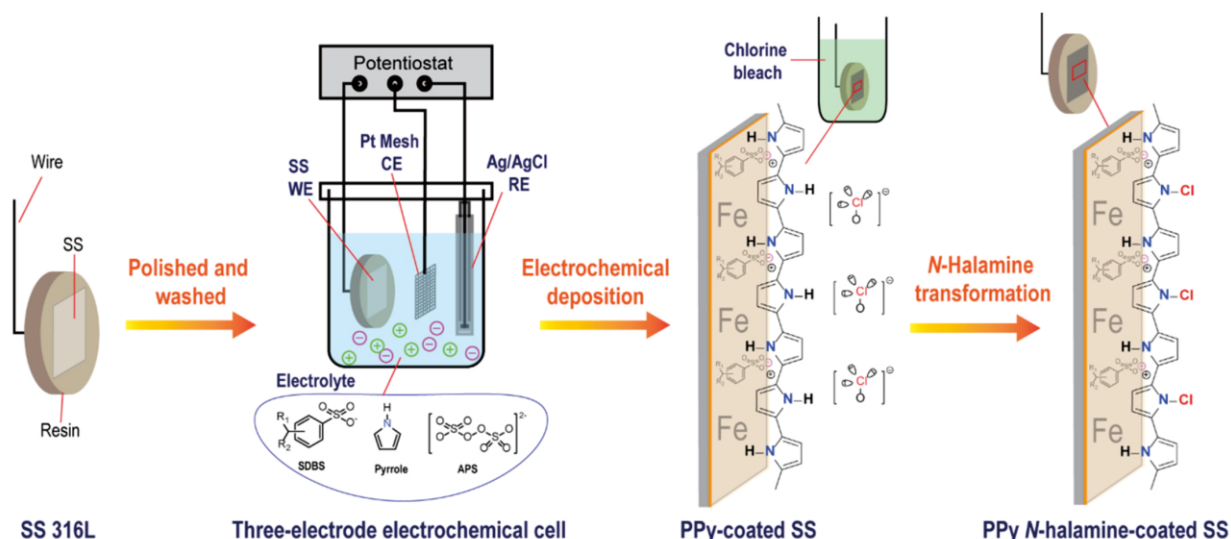
Scheme 1. Illustration of the preparation of PPy N -halamine-coated stainless steel.
