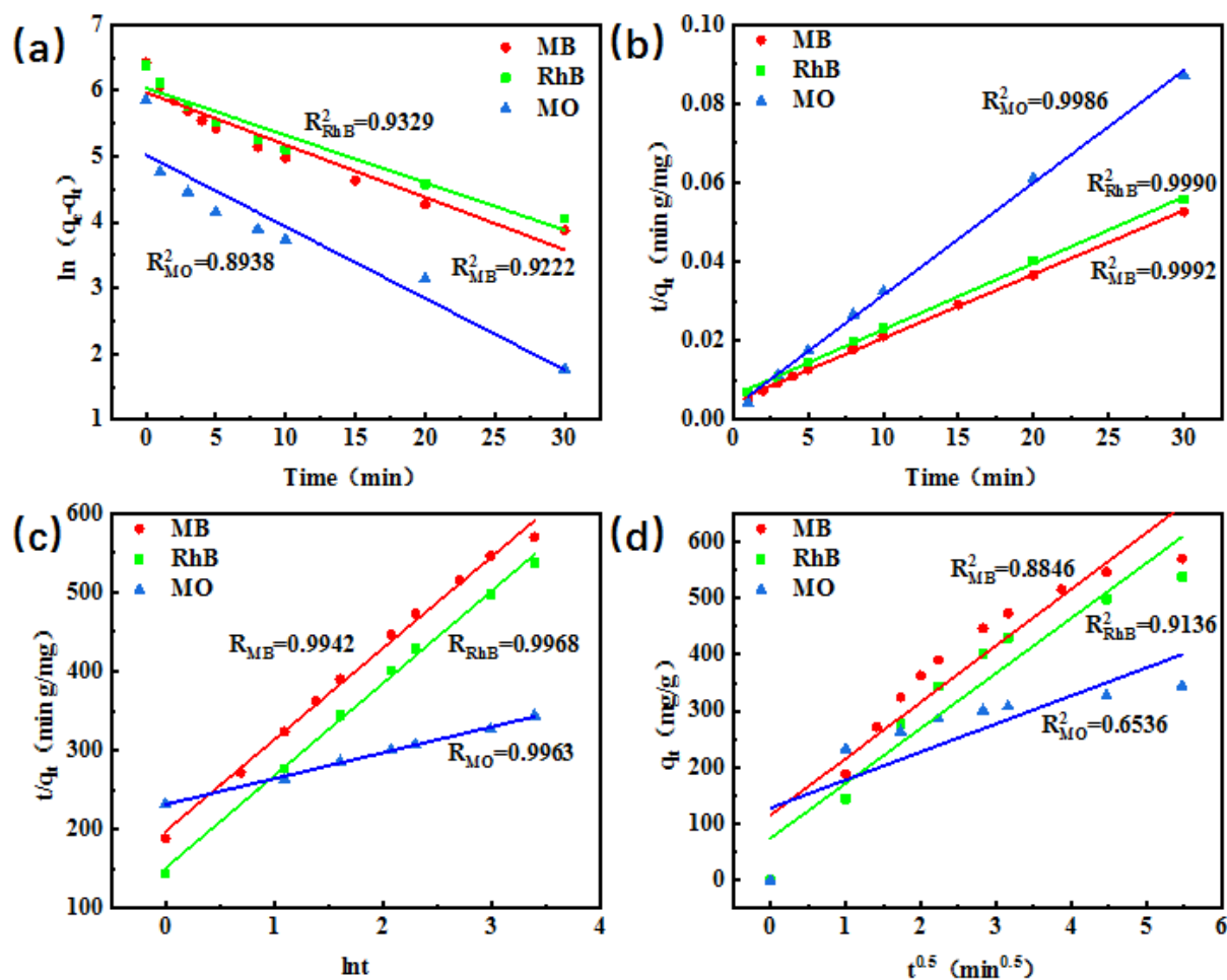
Fig. 5 The kinetics study on the adsorption processes. Plots of (a) \ln(q_e - q_t) against t for pseudo-first order model, (b) t/q_t against t for pseudo-second order model, (c) t/q_t against \ln t for Elovich model and (d) q_t against t^{0.5} for intra-particle diffusion model.
