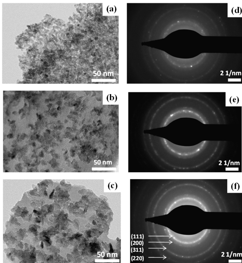
Fig. 5 TEM images of ZrO_2 thin films on glass substrate at 450 °C. Deposition condition (concentration of precursor solution): (a) 0.05 M; (b) 0.075 M; (c) 0.1 M. The Corresponding SAED patterns: (d) 0.05 M; (e) 0.075 M; (f) 0.1 M.
