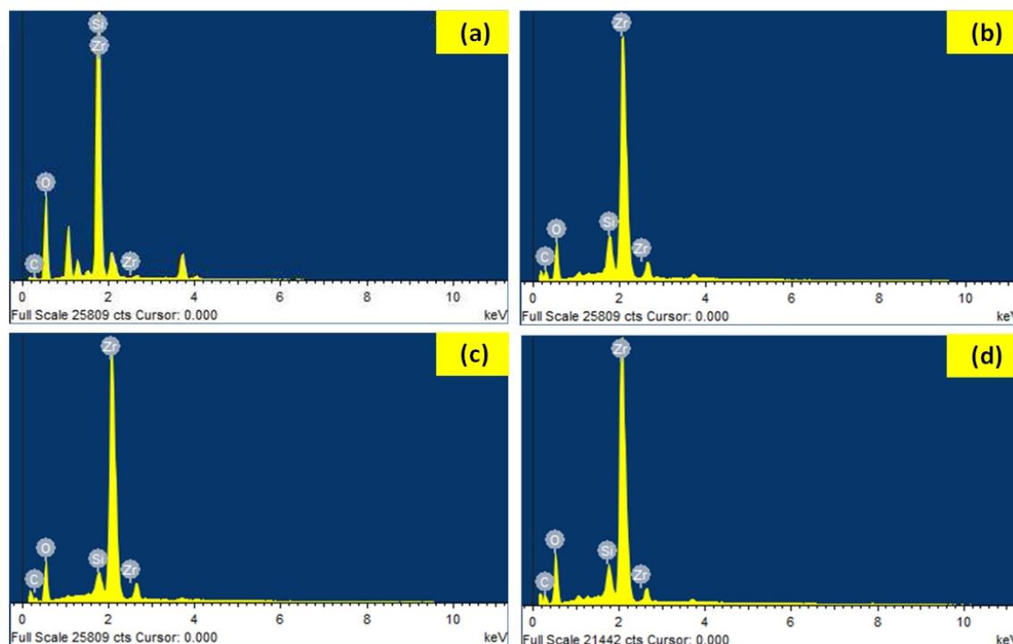
Fig. 4 EDX spectra of ZrO_2 thin films on glass substrate. Deposition condition (concentration of precursor solution): (a) 0.025 M; (b) 0.05 M; (c) 0.075 M; (d) 0.1 M.
