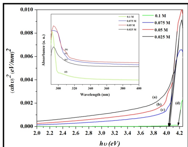
Fig. 6 Variation of (ahv)^2 versus hv of ZrO 2 thin films deposited onto glass substrate at 450 °C: (a) 0.025 M, (b) 0.05 M, (c) 0.075 M, (d) 0.1 M. The inset shows variation in absorbance with wavelength of ZrO 2 thin films: (a) 0.025 M, (b) 0.05 M, (c) 0.075 M, (d) 0.1 M.
