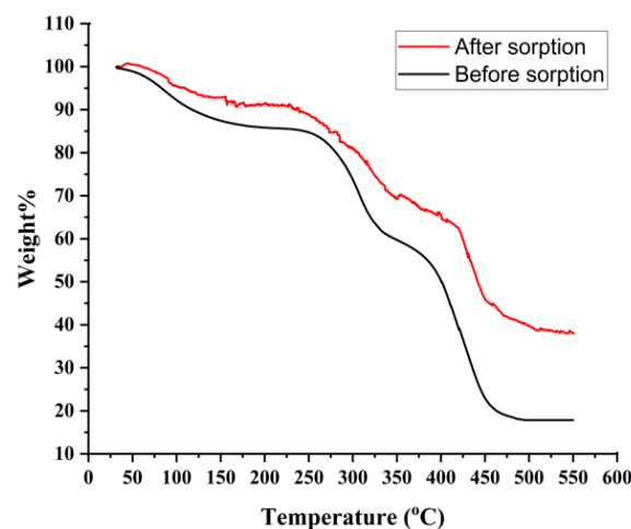
Fig. 10: TGA of initial Amberlite IR120 and Amberlite IR120 from the interpolpolymer system "Amberlite IR120:AV-17-8" (4:2).
