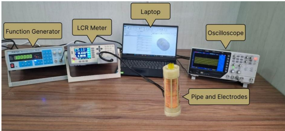
Fig. S1: The experimental setup designed to measure the capacitance values of an 8-blade concave sensor.
